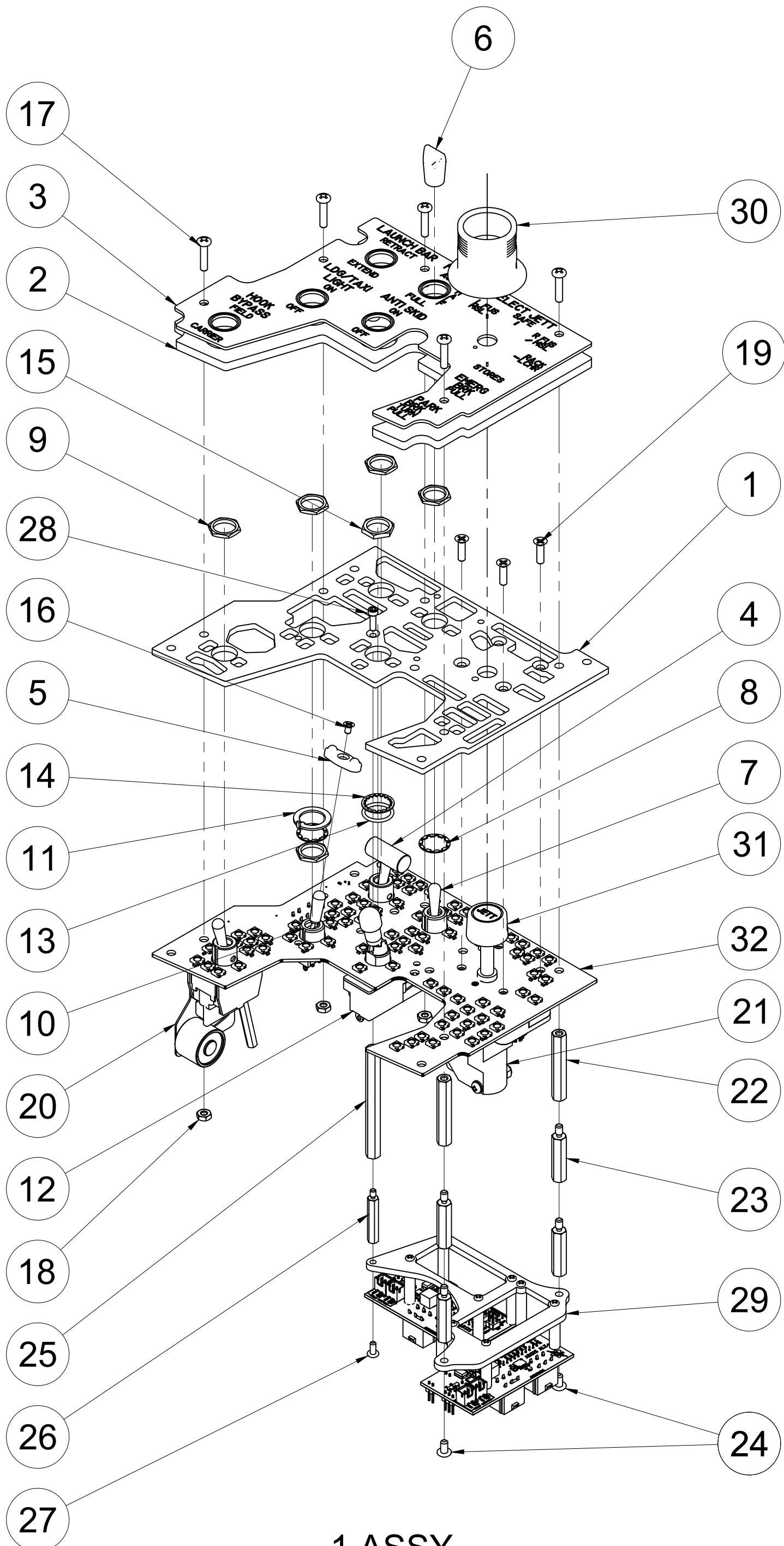
-1 ASSY
