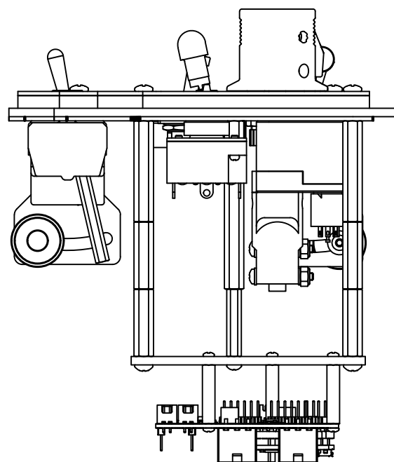
-1 SIDE
