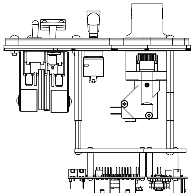
-1 FRONT
